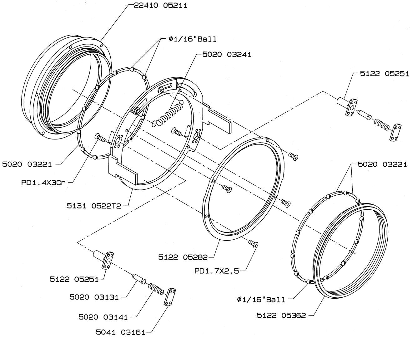
DETAIL D
