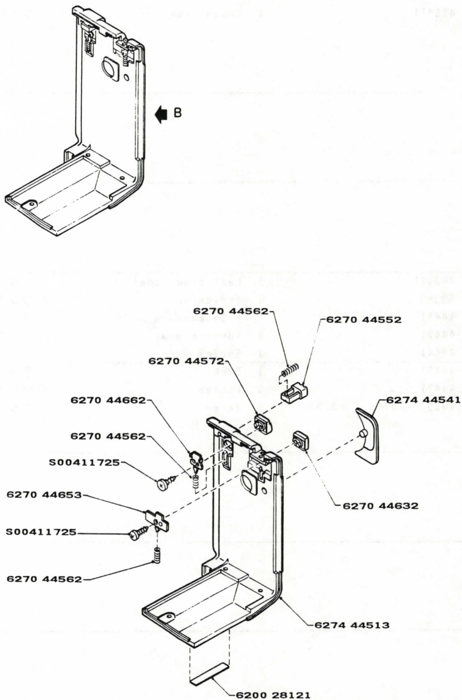
DETAIL B
