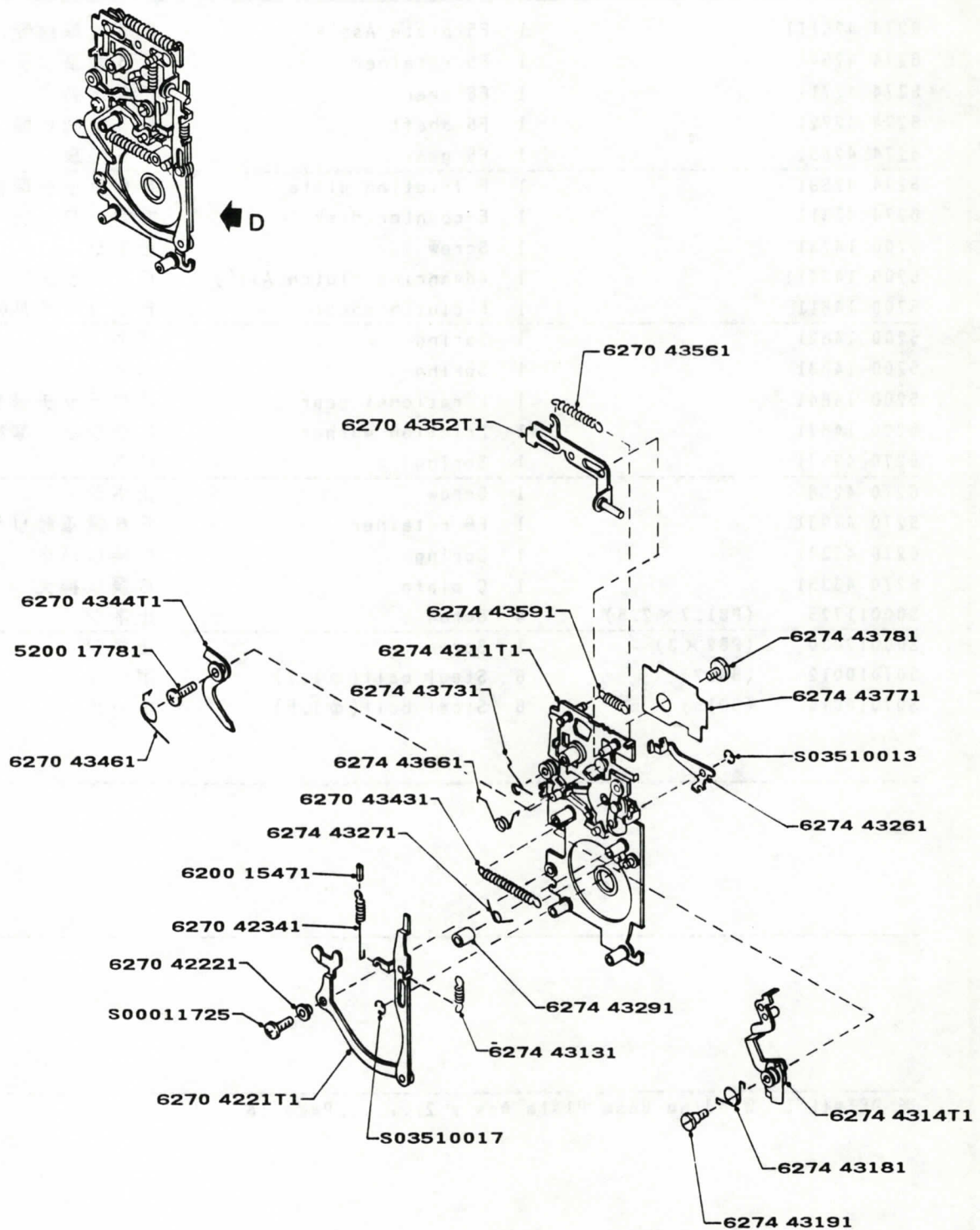
DETAIL D
