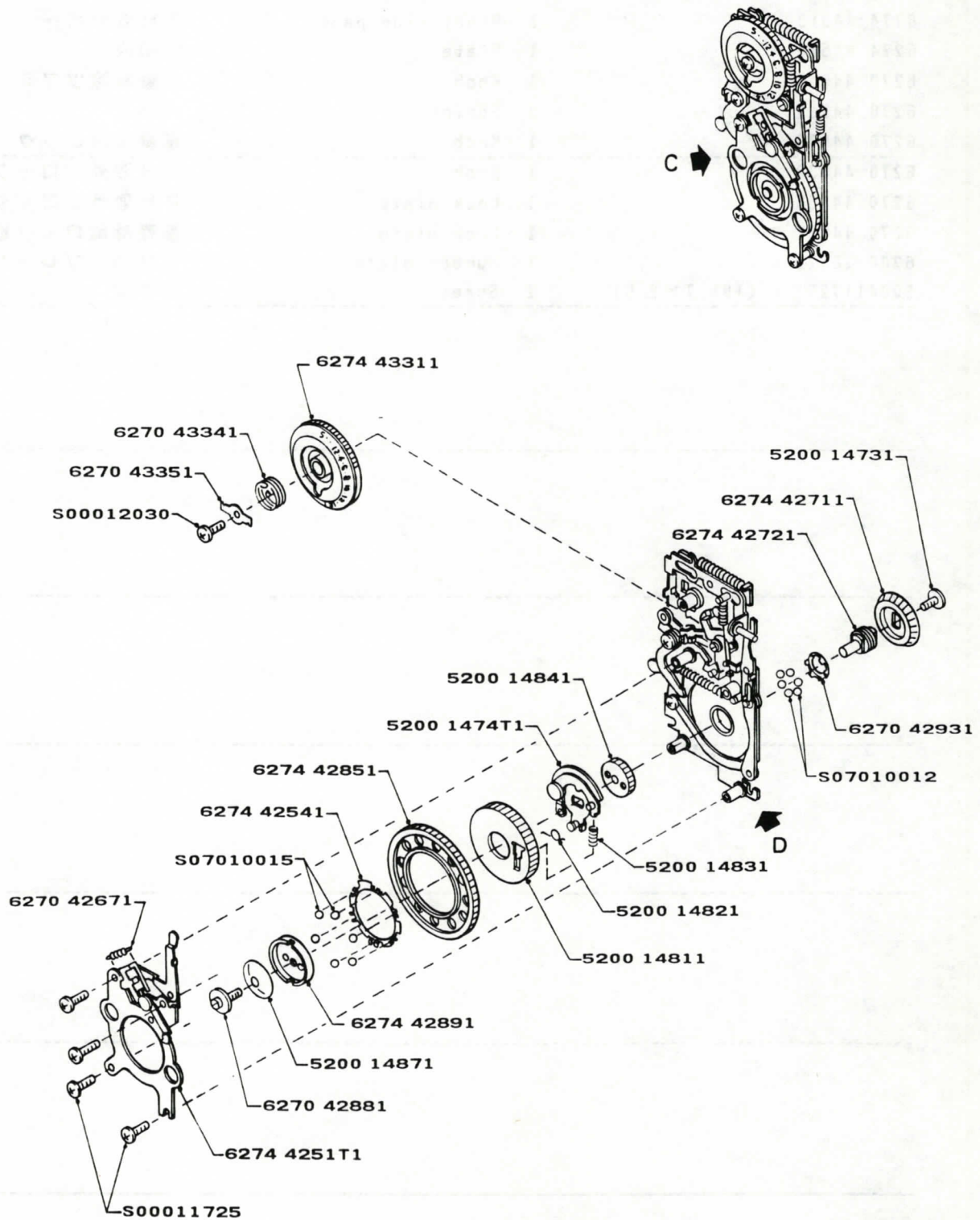
DETAIL C
