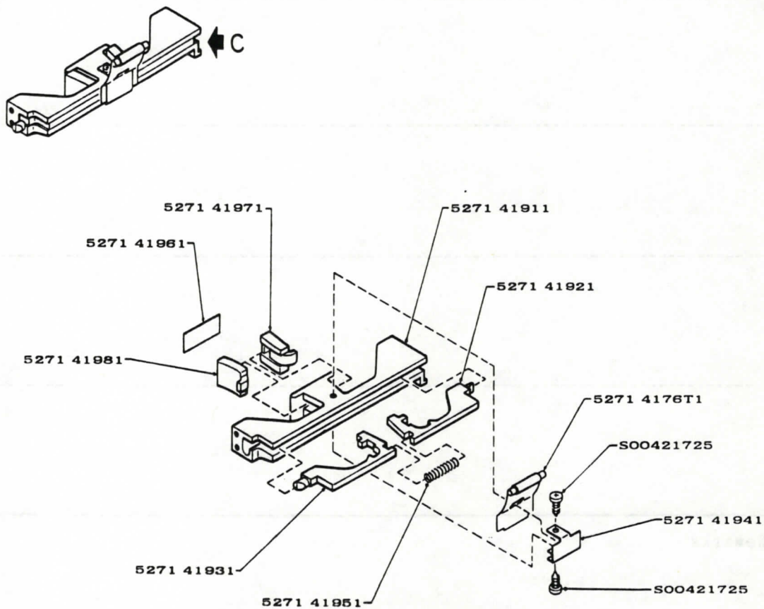
DETAIL "C"
