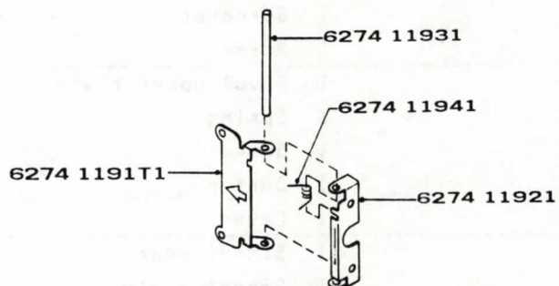
DETAIL E
