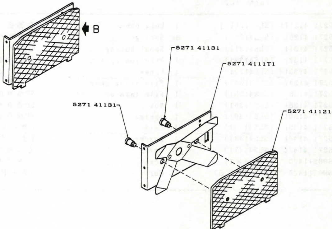
DETAIL "B"
