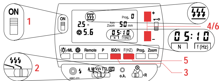
Fig. 19: Settings for stroboscopic mode
