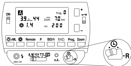
Fig. 27: Automatic cut-out
