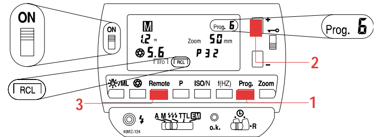
Fig. 22: Calling a stored user program
