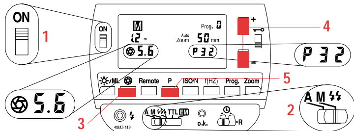
Fig. 17: Partial light output levels in the manual mode
