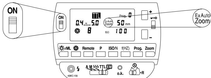
Fig. 23: Settings for Ex-Zoom mode
